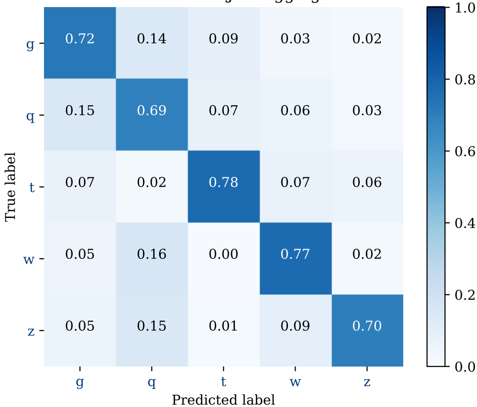
Confusion Matrix of a Jet Tagging Classifier
